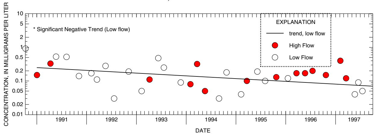
Figure A-4. Relation of total ammonia + organic nitrogen concentrations and load to streamflow and trends in low and high-flow concentrations at 01396660 Mulhockaway Creek near Van Syckel, NJ
