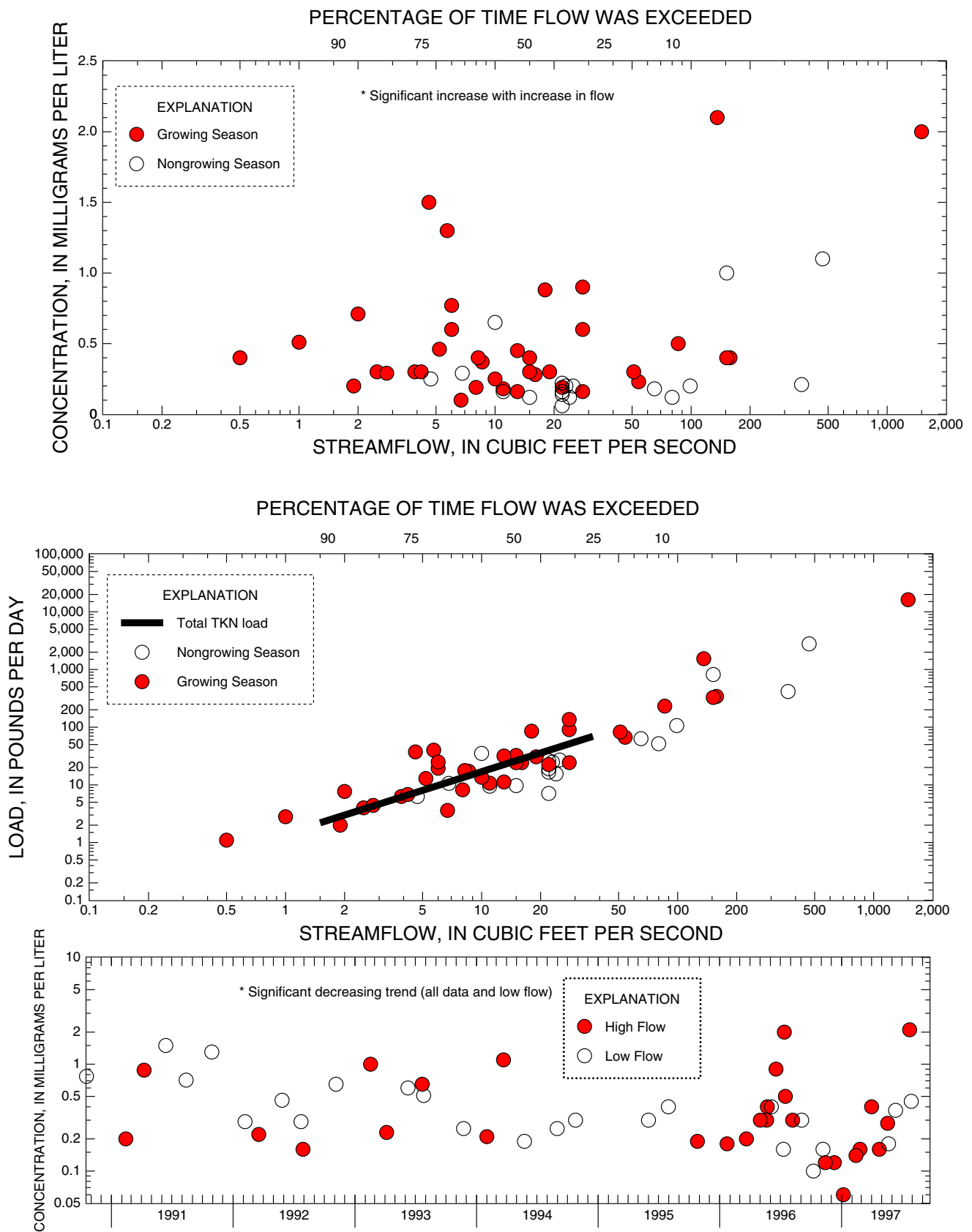
Figure A-7. Relation of total ammonia + organic nitrogen concentrations and load to streamflow and trends in low and high-flow concentrations at 01398000 Neshanic River at Reaville, NJ
