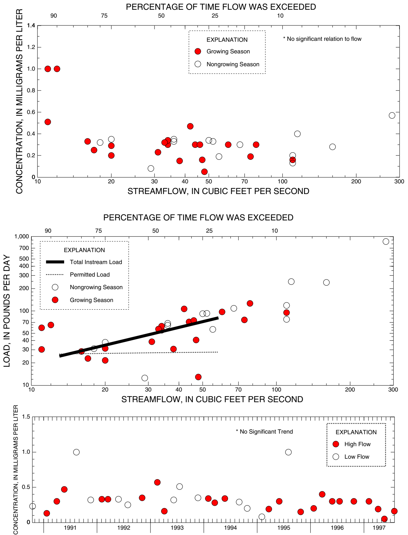
Figure A-11. Relation of total ammonia plus organic nitrogen concentrations and load to streamflow and trends in low and high-flow concentrations at 01399700 Rockaway Creek at Whitehouse, NJ
