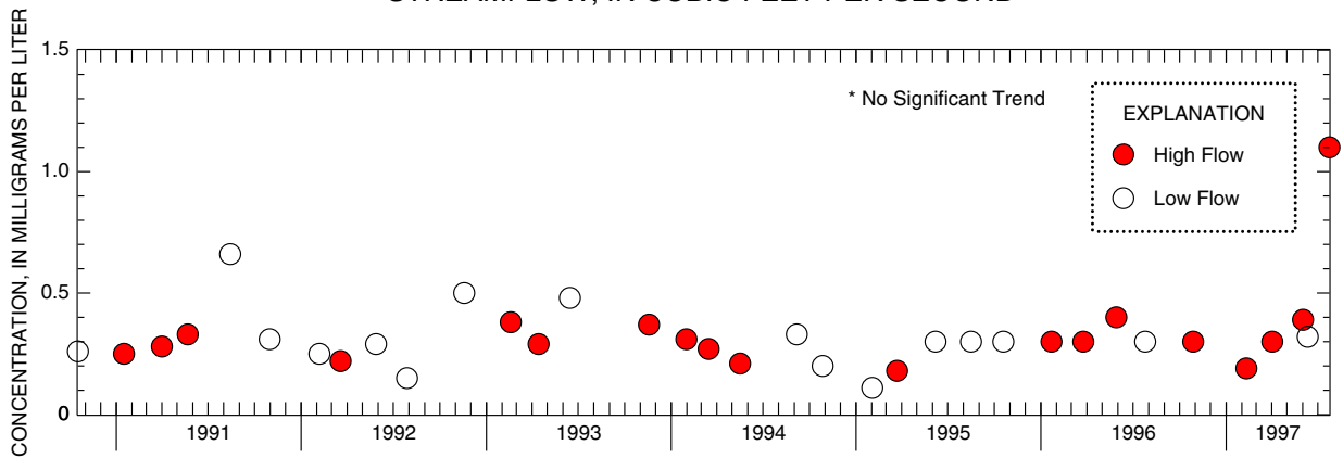
Figure A-12. Relation of total ammonia plus organic nitrogen concentrations and load to streamflow and trends in low and high-flow concentrations at 01399780 Lamington River at Burnt Mills, NJ
