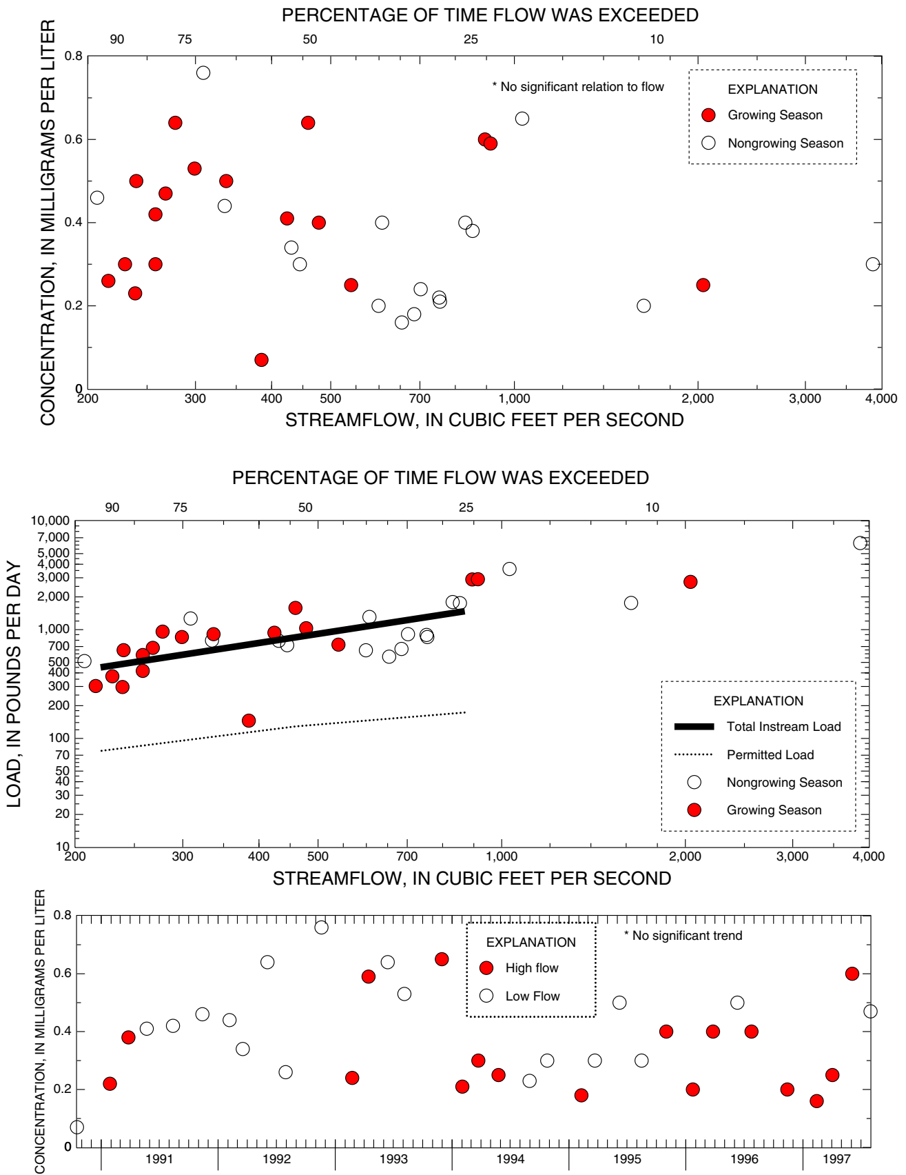
Figure A-13. Relation of total ammonia plus organic nitrogen concentrations and load to streamflow and trends in low and high-flow concentrations at 01400500 Raritan River at Manville, NJ
