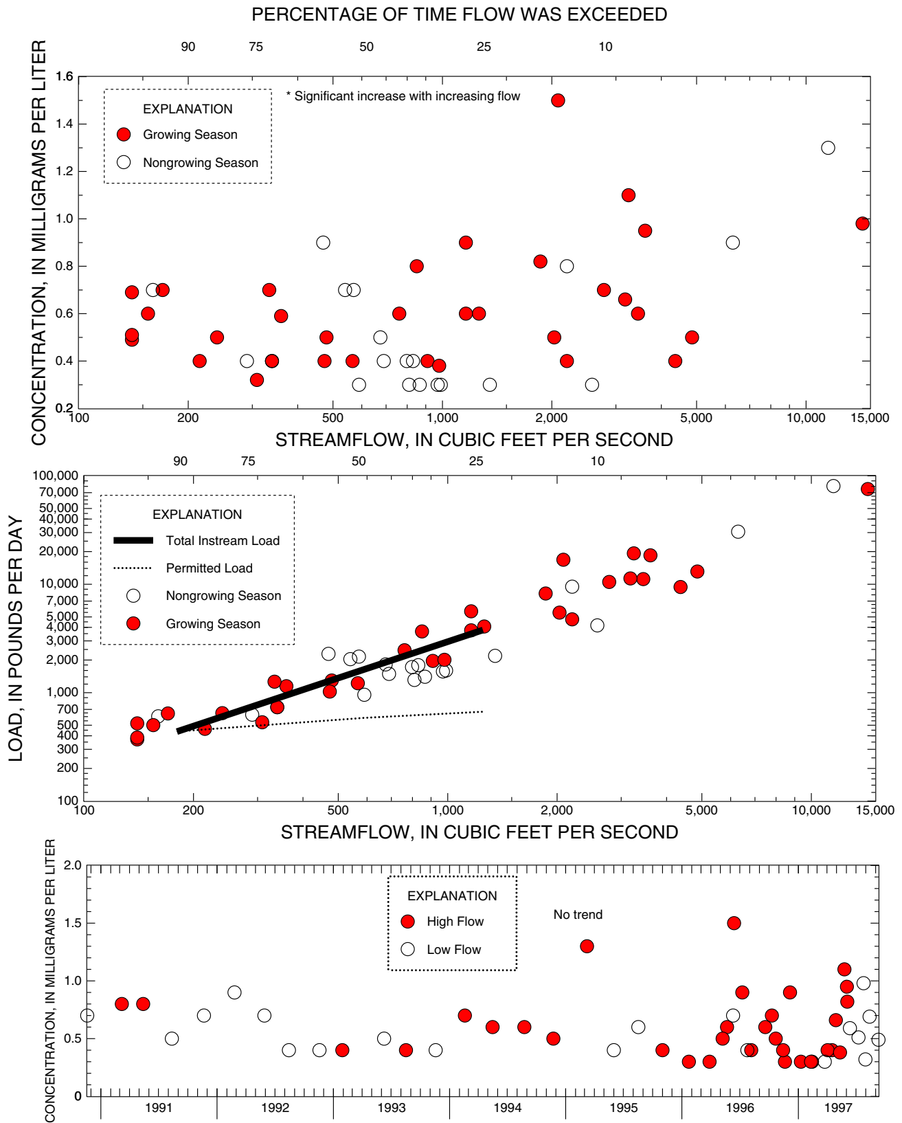
Figure A-19. Relation of total ammonia plus organic nitrogen concentrations and load to streamflow and trends in low and high-flow concentrations at 01403300 Raritan River at Queens Bridge at Bound Brook, NJ
