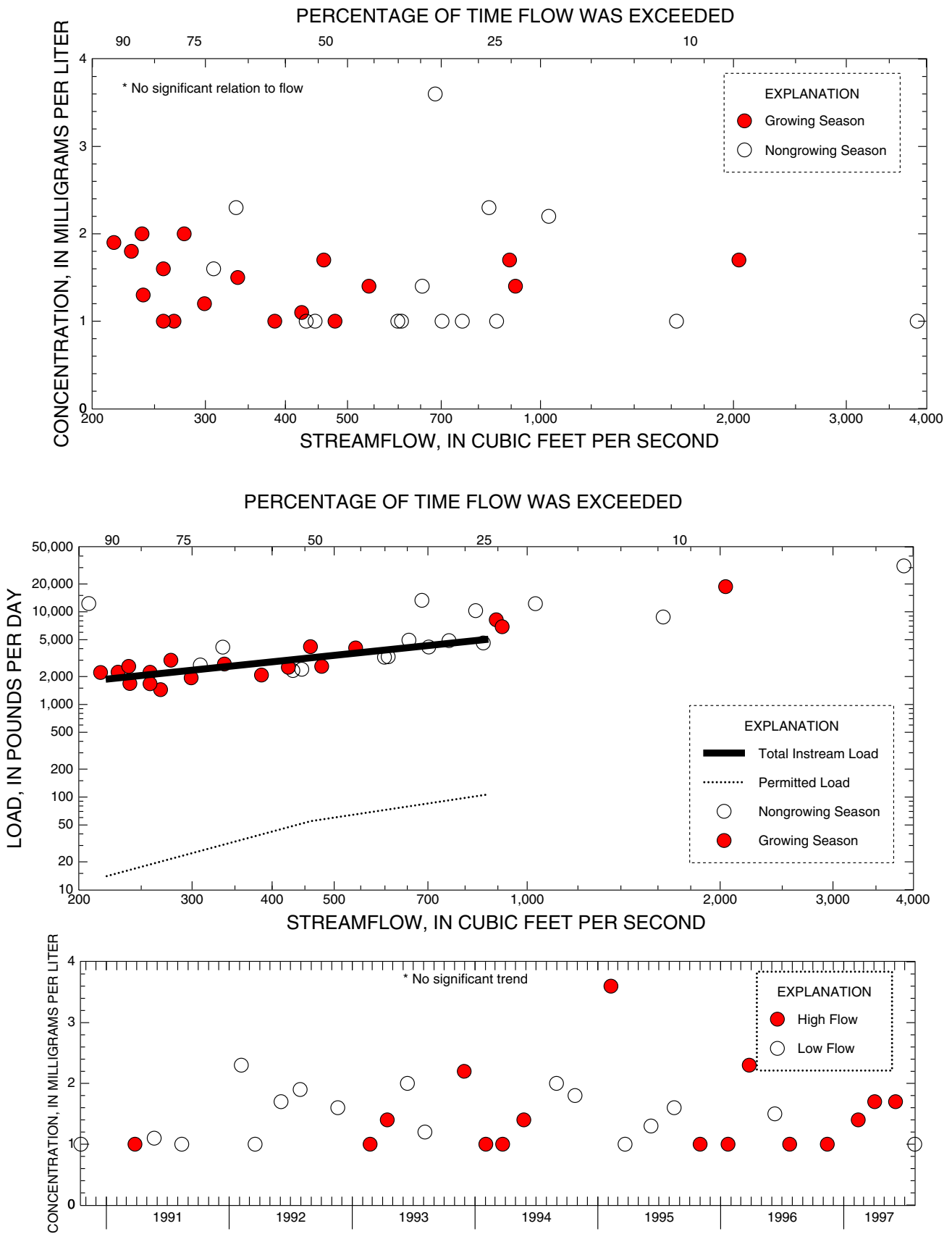
Figure B-13. Relation of biochemical oxygen demand concentrations and load to streamflow and trends in low and high-flow concentrations at 01400500 Raritan River at Manville, NJ
