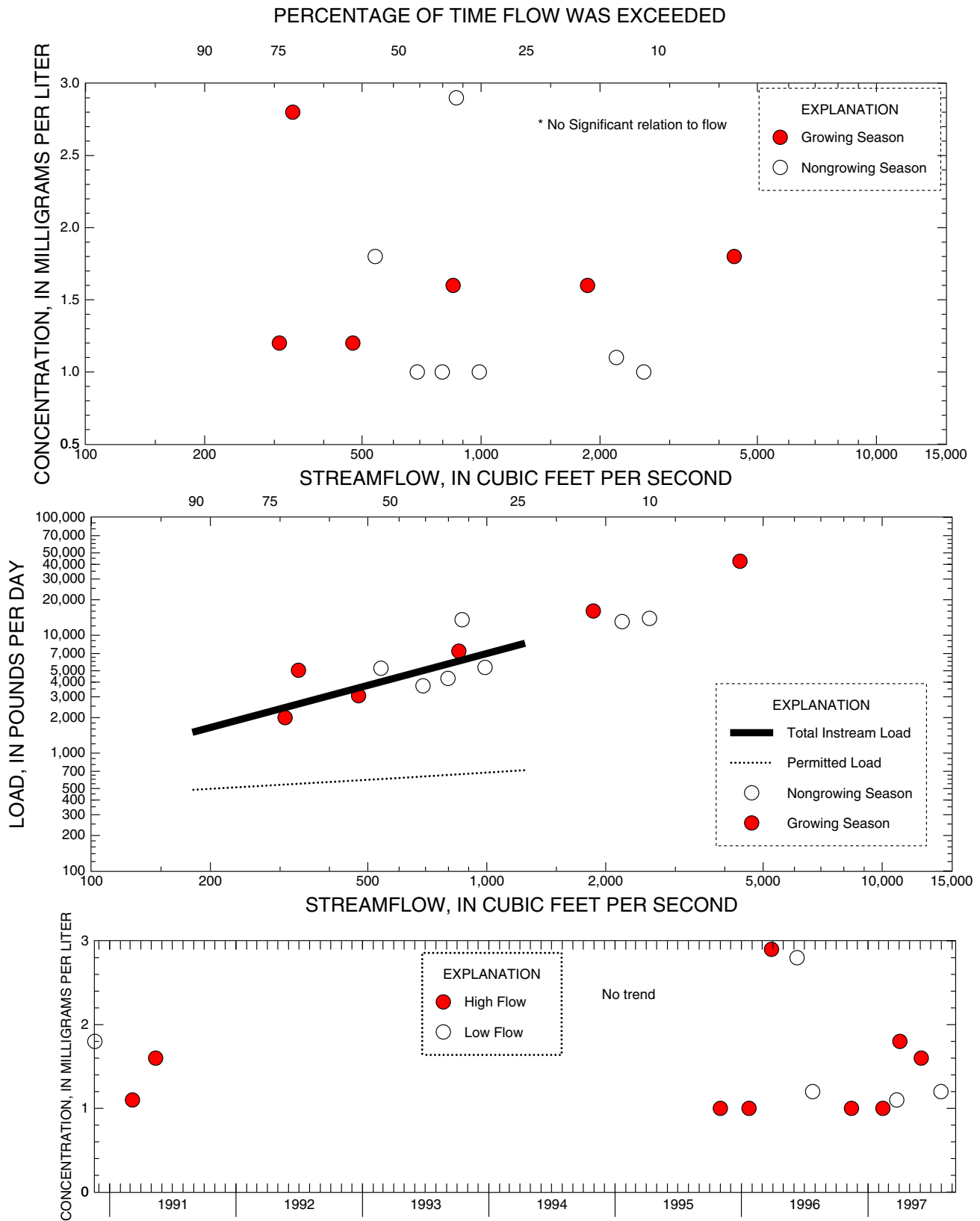
Figure B-19. Relation of biochemical oxygen demand concentrations and load to streamflow and trends in low and high-flow concentrations at 01403300 Raritan River at Queens Bridge at Bound Brook, NJ
