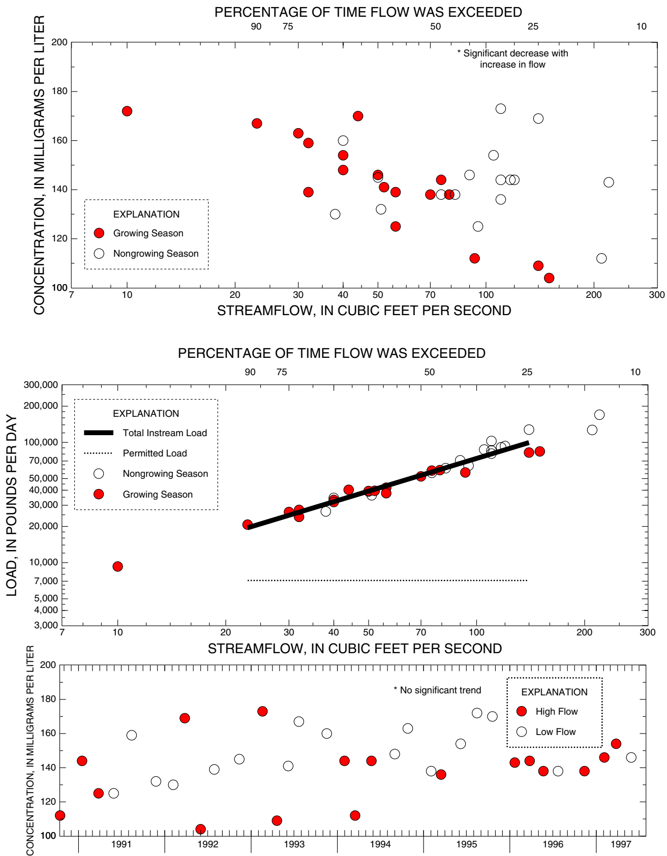
Figure C-9. Relation of total dissolved solids concentrations and load to streamflow and trends in low and high-flow concentrations at 01399120 N.B. Raritan River at Burnt Mills, NJ
