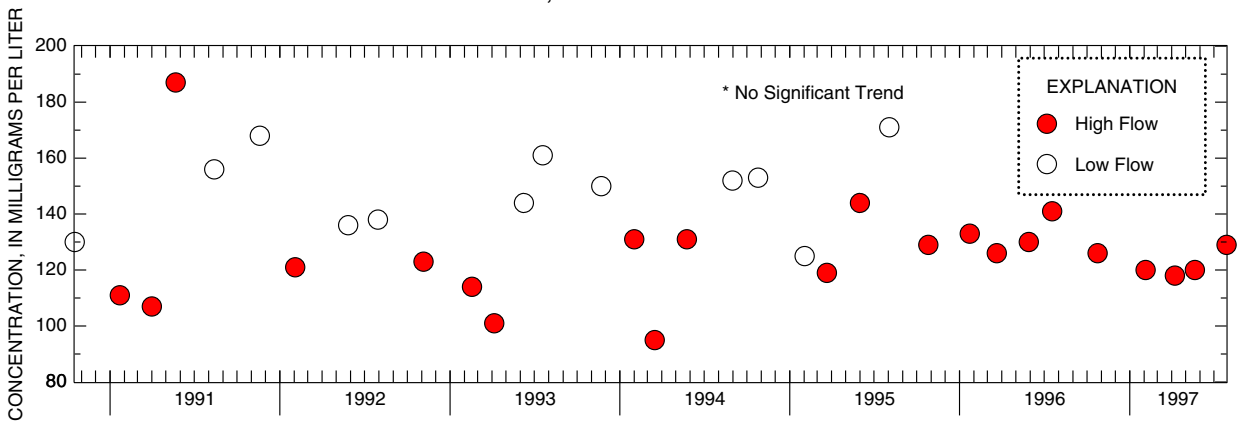
Figure C-11. Relation of total dissolved solids concentrations and load to streamflow and trends in low and high-flow concentrations at 01399700 Rockaway Creek at Whitehouse, NJ
