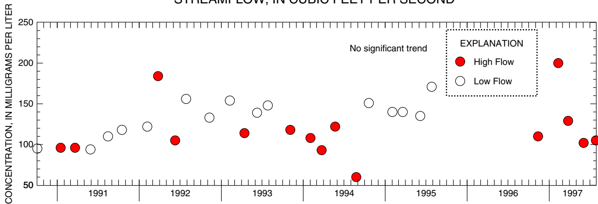
Figure C-15. Relation of total dissolved solids concentrations and load to streamflow and trends in low and high-flow concentrations at 01400650 Millstone River at Grovers Mill, NJ
