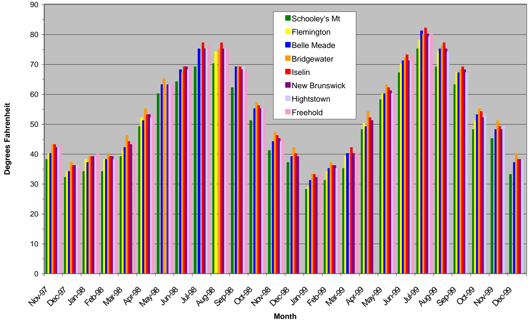
Figure 13 Mean Temperature within the Raritan Basin
