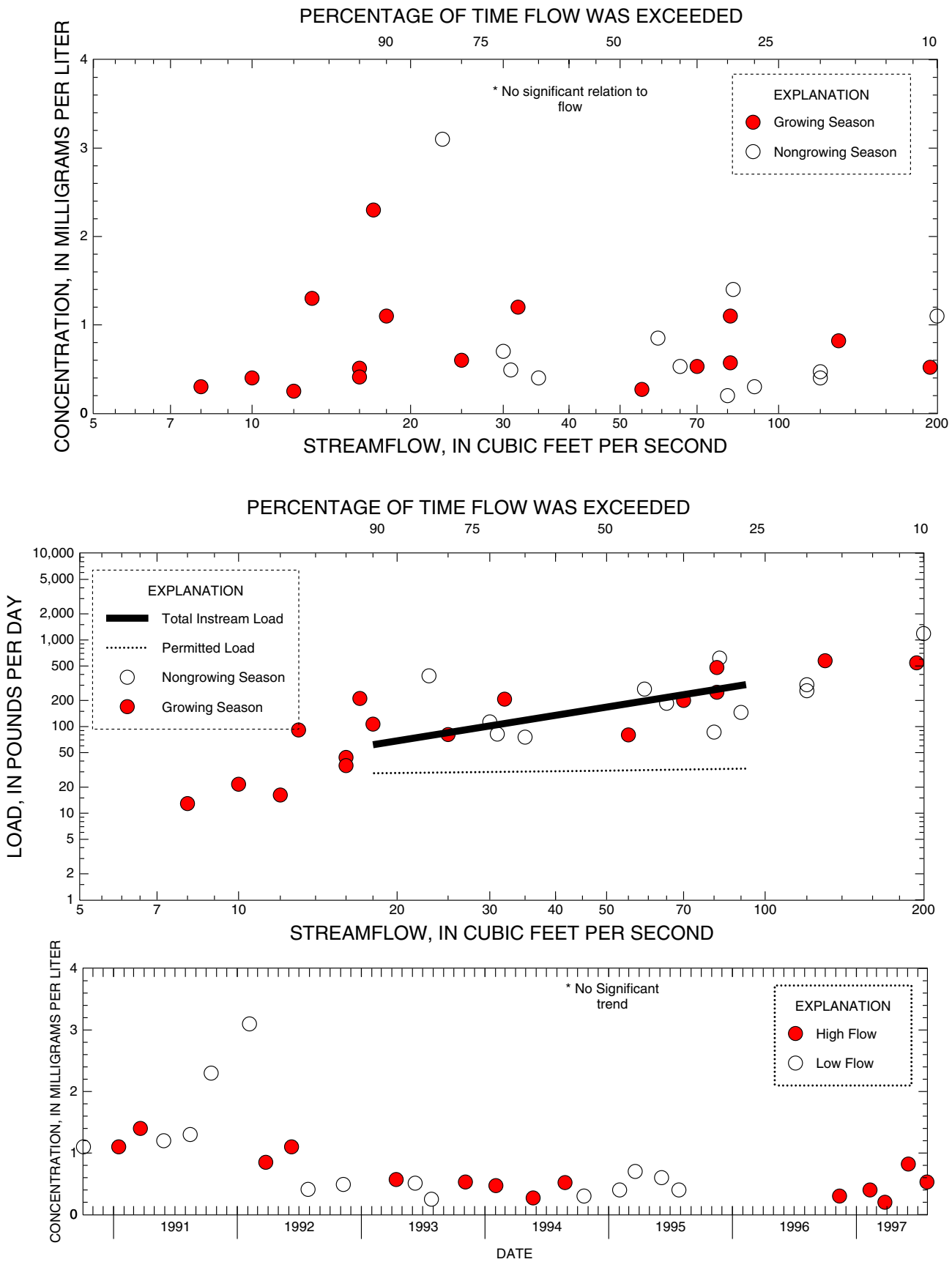
Figure A-15. Relation of total ammonia + organic nitrogen concentrations and load to streamflow and trends in low and high-flow concentrations at 01400650 Millstone River at Grovers Mill, NJ
