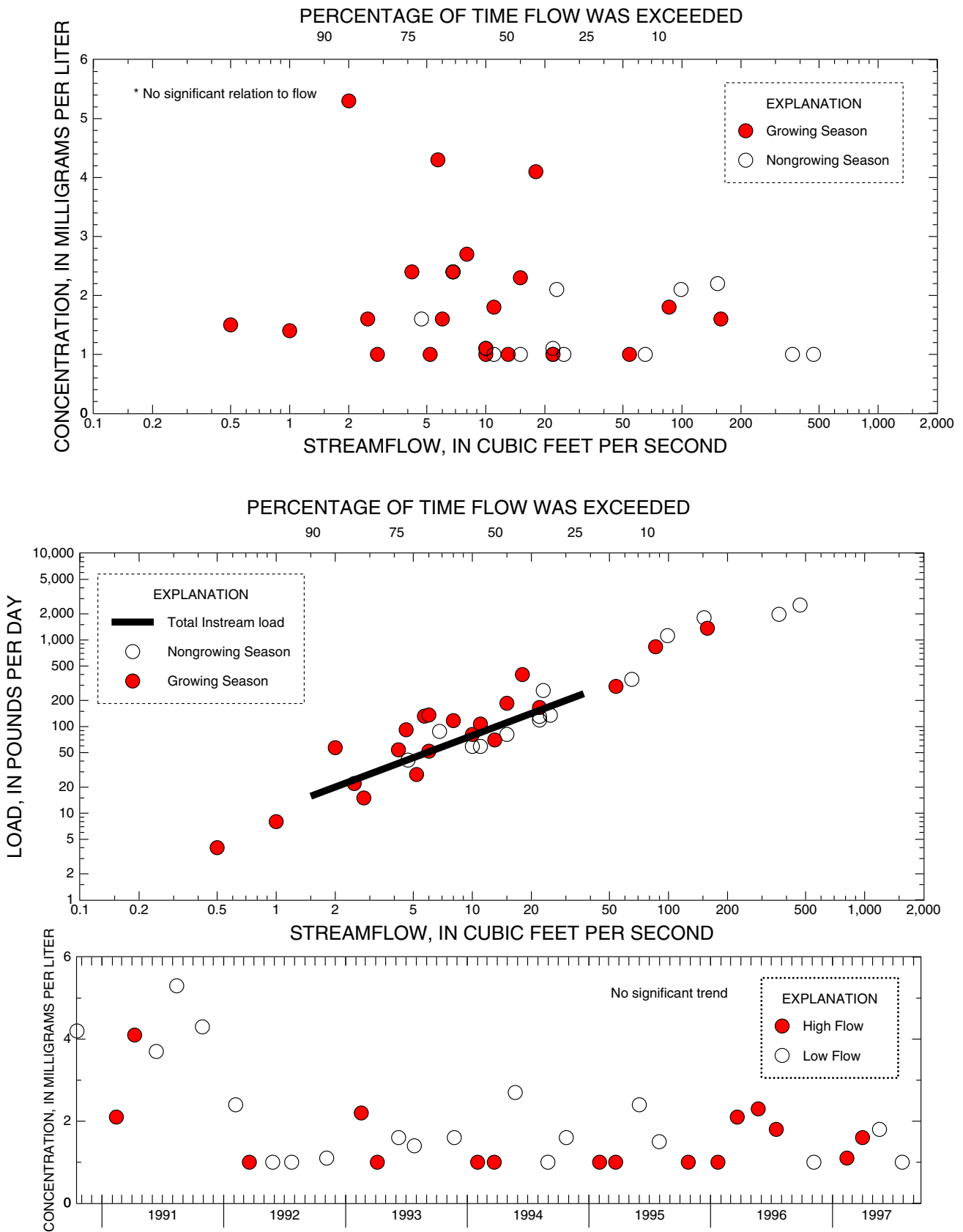
Figure B-7. Relation of biochemical oxygen demand concentrations and load to streamflow and trends in low and high-flow concentrations at 01398000 Neshanic River at Reaville, NJ
