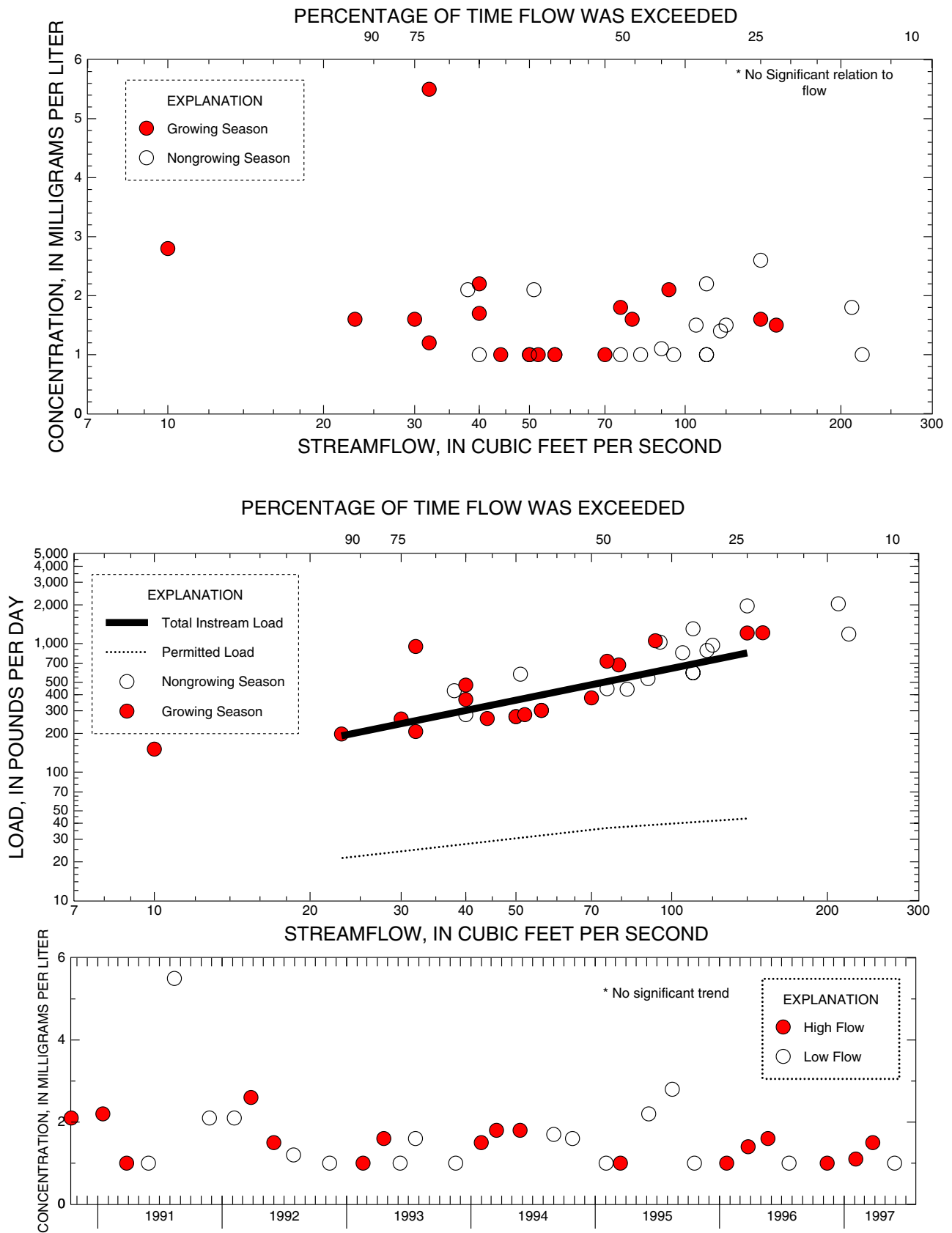
Figure B-9. Relation of biochemical oxygen demand concentrations and load to streamflow and trends in low and high-flow concentrations at 01399120 N.B. Raritan River at Burnt Mills, NJ
