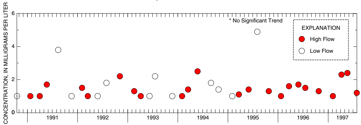
Figure B-11. Relation of biochemical oxygen demand concentrations and load to streamflow and trends in low and high-flow concentrations at 01399700 Rockaway Creek at Whitehouse, NJ
