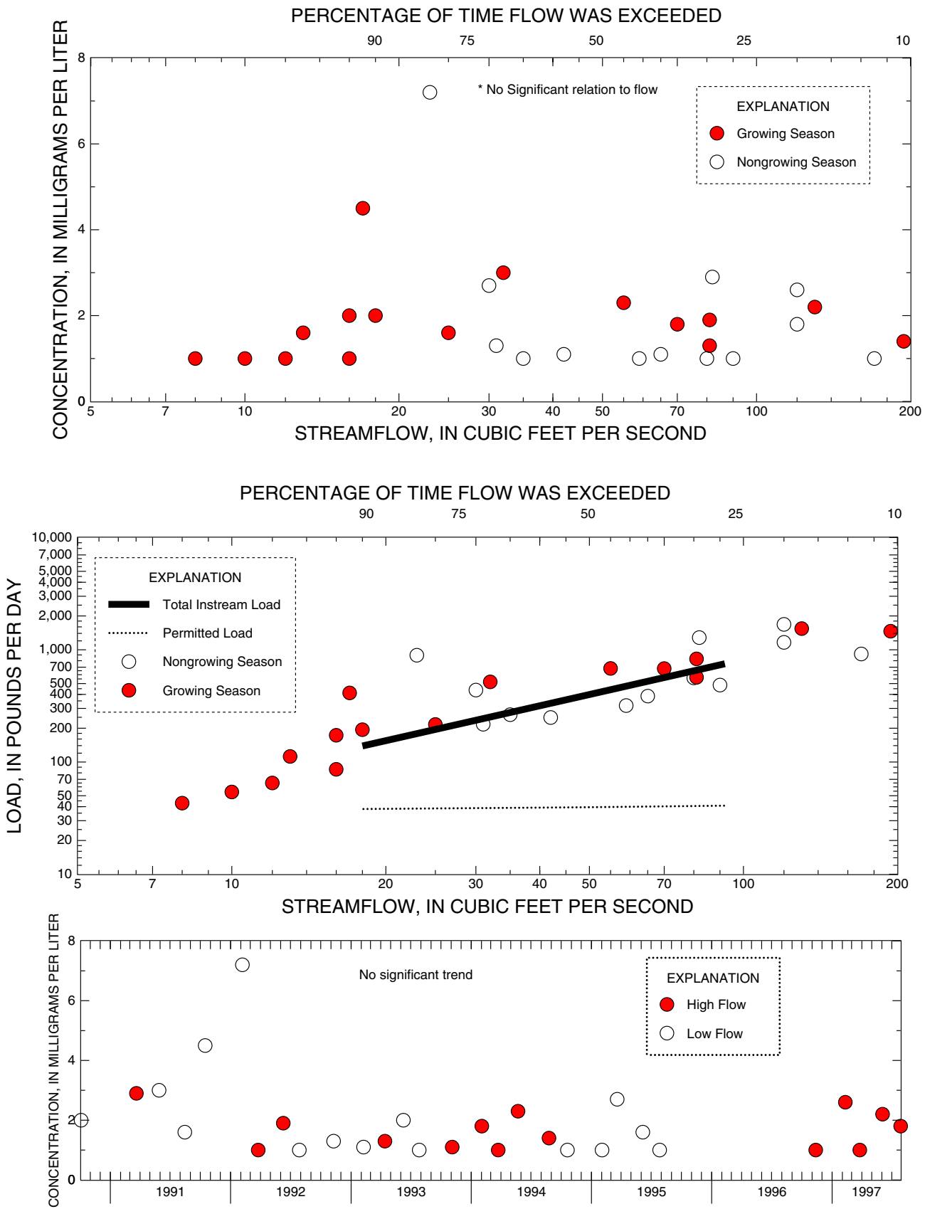
Figure B-15. Relation of biochemical oxygen demand concentrations and load to streamflow and trends in low and high-flow concentrations at 01400650 Millstone River at Grovers Mill, NJ
