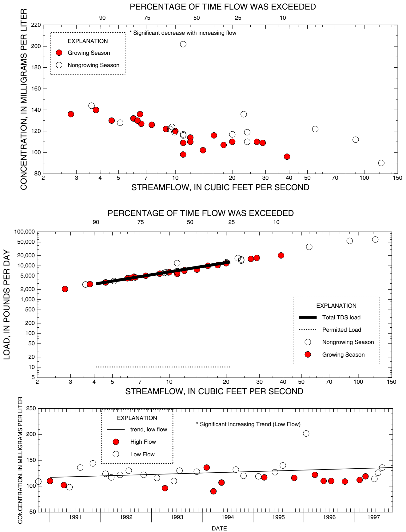
Figure C-4. Relation of total dissolved solids concentrations and load to streamflow and trends in low and high-flow concentrations at 01396660 Mulhockaway Creek near Van Syckel, NJ
