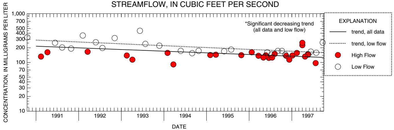
Figure C-7. Relation of total dissolved solids concentrations and load to streamflow and trends in low and high-flow concentrations at 01398000 Neshanic River at Reaville, NJ
