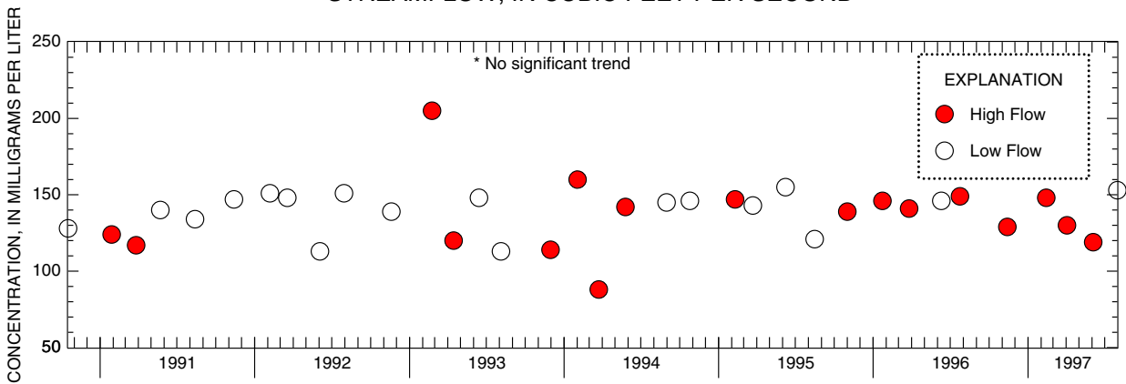
Figure C-13. Relation of total dissolved solids concentrations and load to streamflow and trends in low and high-flow concentrations at 01400500 Raritan River at Manville, NJ
