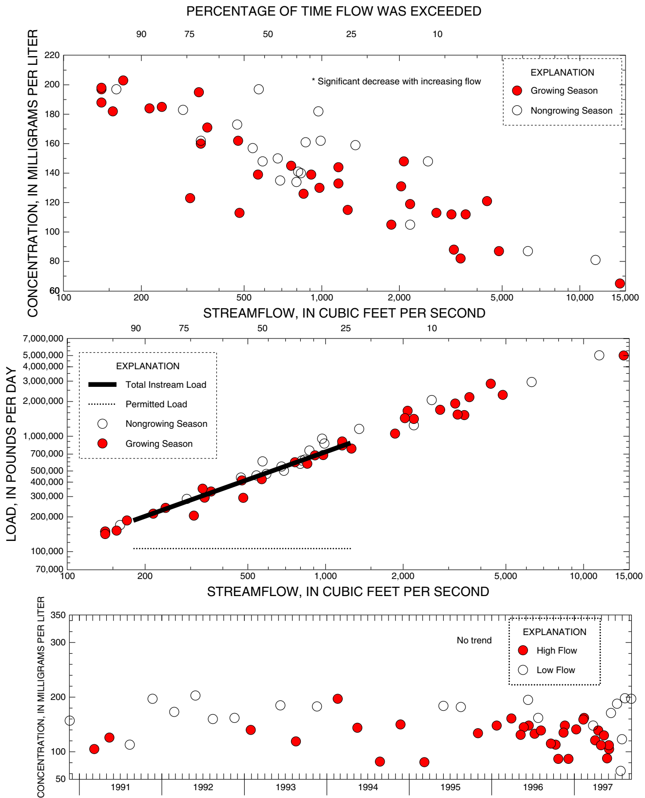
Figure C-19. Relation of total dissolved solids concentrations and load to streamflow and trends in low and high-flow concentrations at 01403300 Raritan River at Queens Bridge at Bound Brook, NJ
