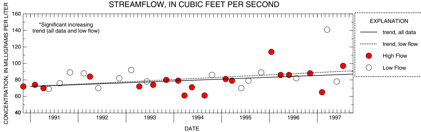
Figure C-21. Relation of total dissolved solids concentrations and load to streamflow and trends in low and high-flow concentrations at 01405340 Manalapan Brook at Federal Road at Manalapan, NJ
