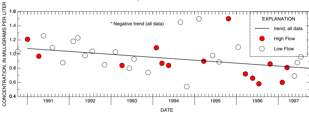
Figure D-4. Relation of nitrate plus nitrite concentrations and load to streamflow and trends in low and high-flow concentrations at 01396660 Mulhockaway Creek near Van Syckel, NJ
