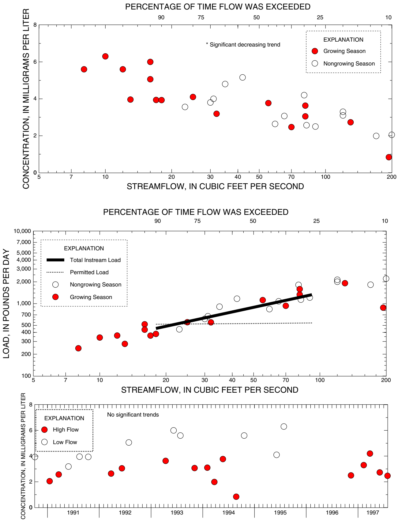
Figure D-15. Relation of nitrate + nitrite concentrations and load to streamflow and trends in low and high-flow concentrations at 01400650 Millstone River at Grovers Mill, NJ
