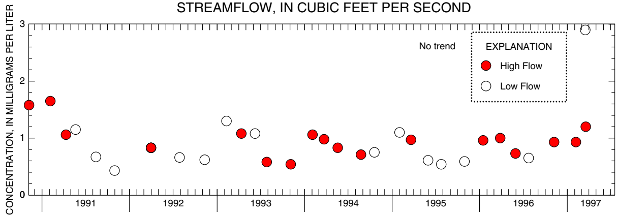
Figure D-21. Relation of nitrate + nitrite concentrations and load to streamflow and trends in low and high-flow concentrations at 01405340 Manalapan Brook at Federal Road at Manalapan, NJ
