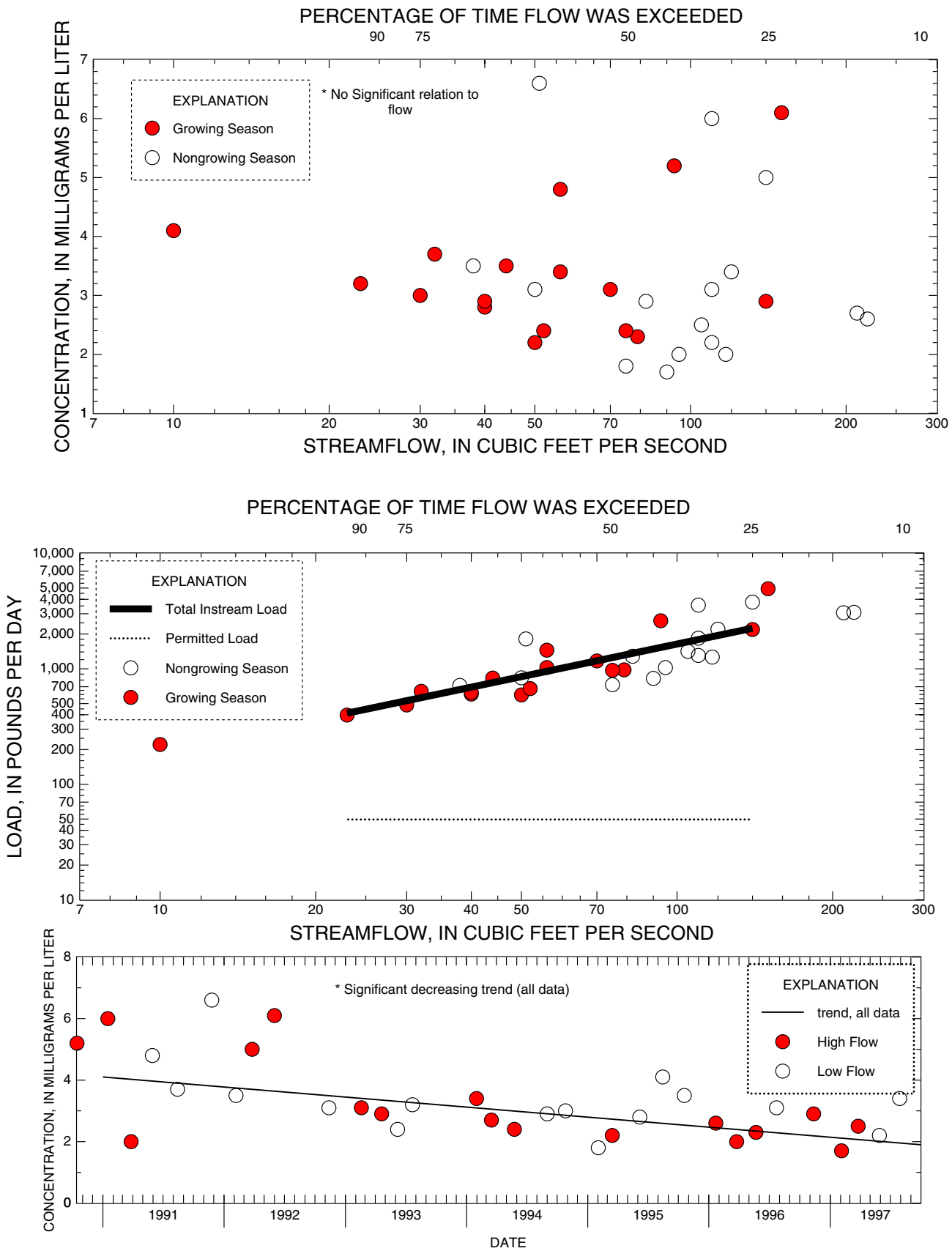
Figure E-9. Relation of total organic carbon concentrations and load to streamflow and trends in low and high-flow concentrations at 01399120 N.B. Raritan River at Burnt Mills, NJ
