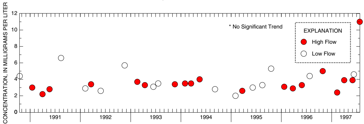
Figure E-12. Relation of total organic carbon concentrations and load to streamflow and trends in low and high-flow concentrations at 01399780 Lamington River at Burnt Mills, NJ
