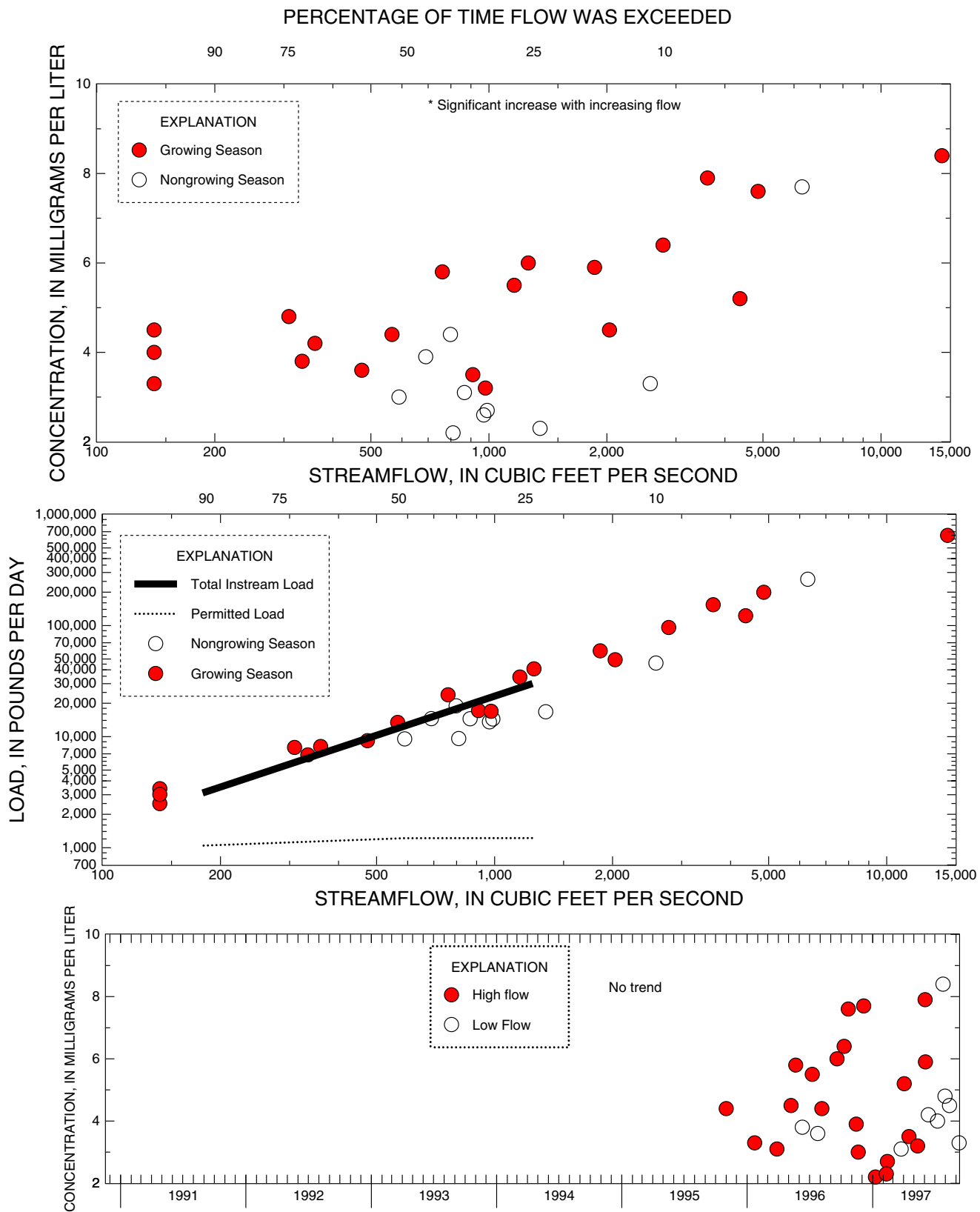
Figure E-19. Relation of total organic carbon concentrations and load to streamflow and trends in low and high-flow concentrations at 01403300 Raritan River at Queens Bridge at Bound Brook, NJ
