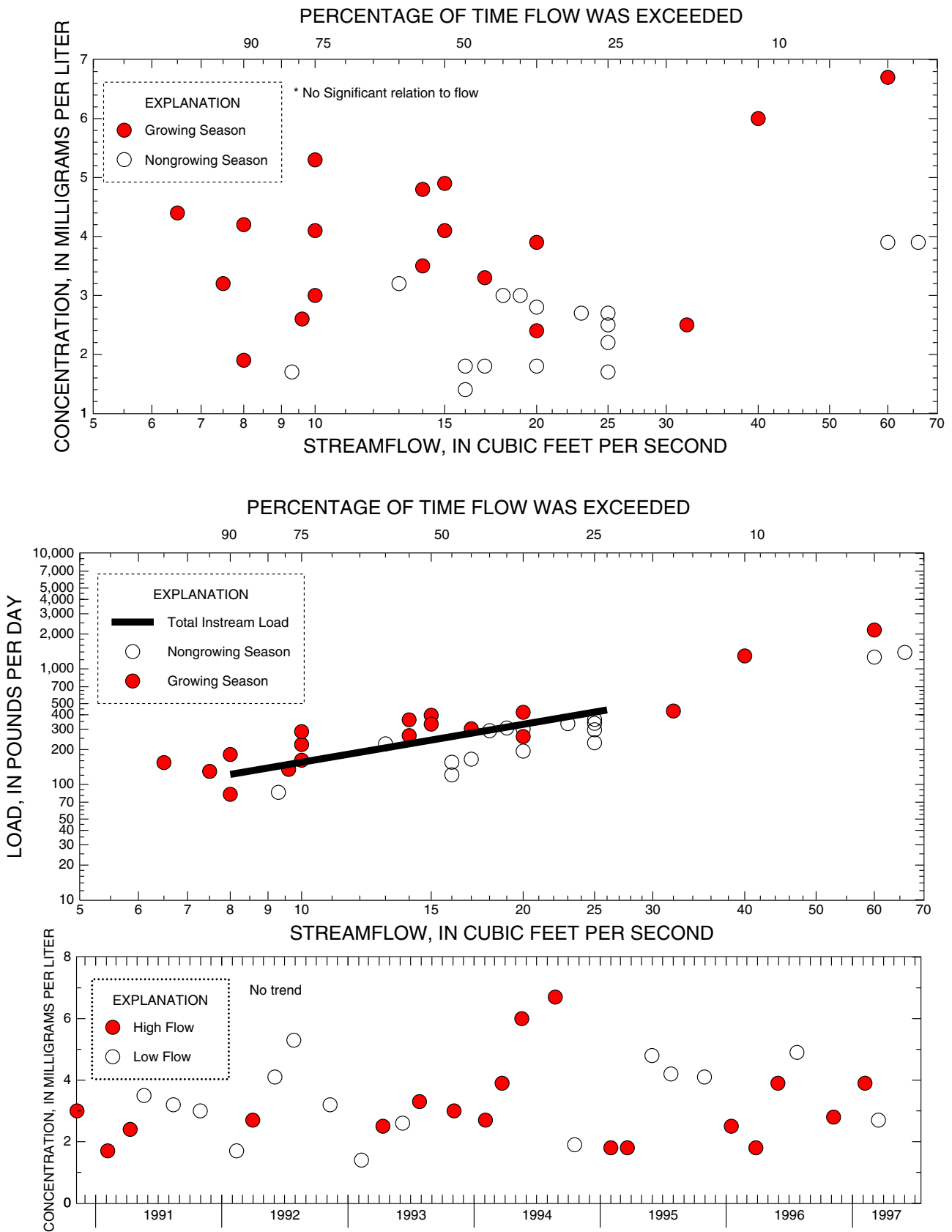
Figure E-21. Relation of total organic carbon concentrations and load to streamflow and trends in low and high-flow concentrations at 01405340 Manalapan Brook at Federal Road at Manalapan, NJ
