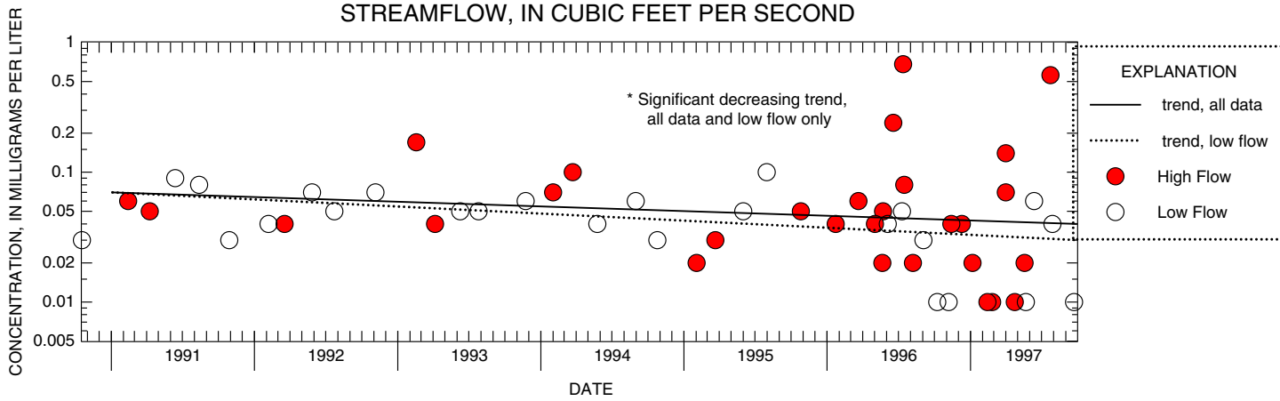
Figure F-7. Relation of total phosphorus concentrations and load to streamflow and trends in low and high-flow concentrations at 01398000 Neshanic River at Reaville, NJ
