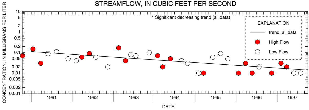
Figure F-9. Relation of total phosphorus concentrations and load to streamflow and trends in low and high-flow concentrations at 01399120 N.B. Raritan River at Burnt Mills, NJ
