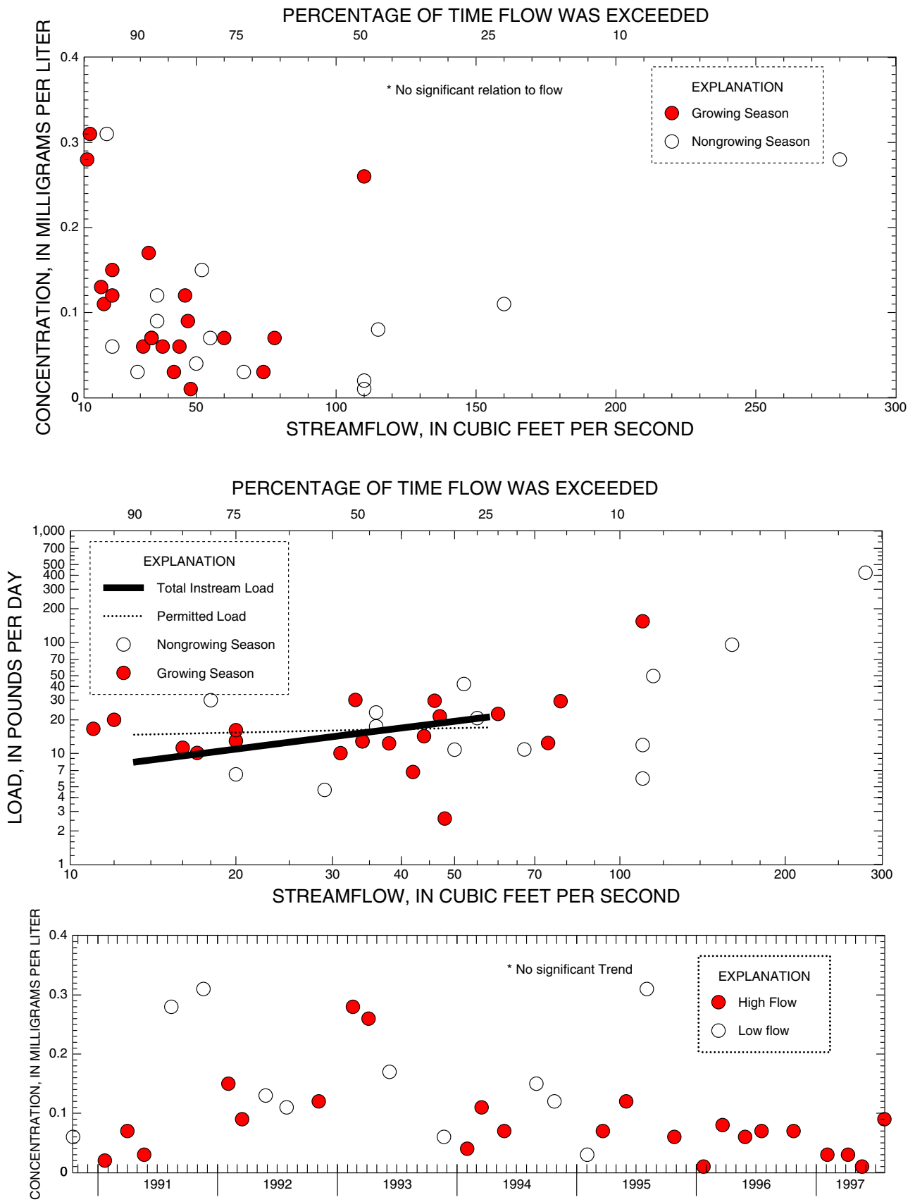
Figure F-11. Relation of total phosphorus concentrations and load to streamflow and trends in low and high-flow concentrations at 01399700 Rockaway Creek at Whitehouse, NJ
