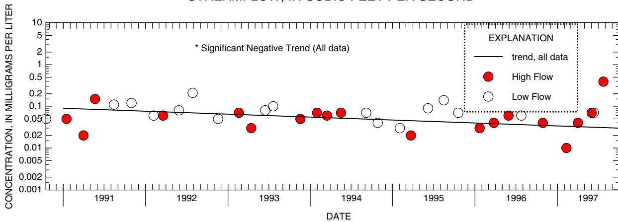
Figure F-12. Relation of total phosphorus concentrations and load to streamflow and trends in low and high-flow concentrations at 01399780 Lamington River at Burnt Mills, NJ
