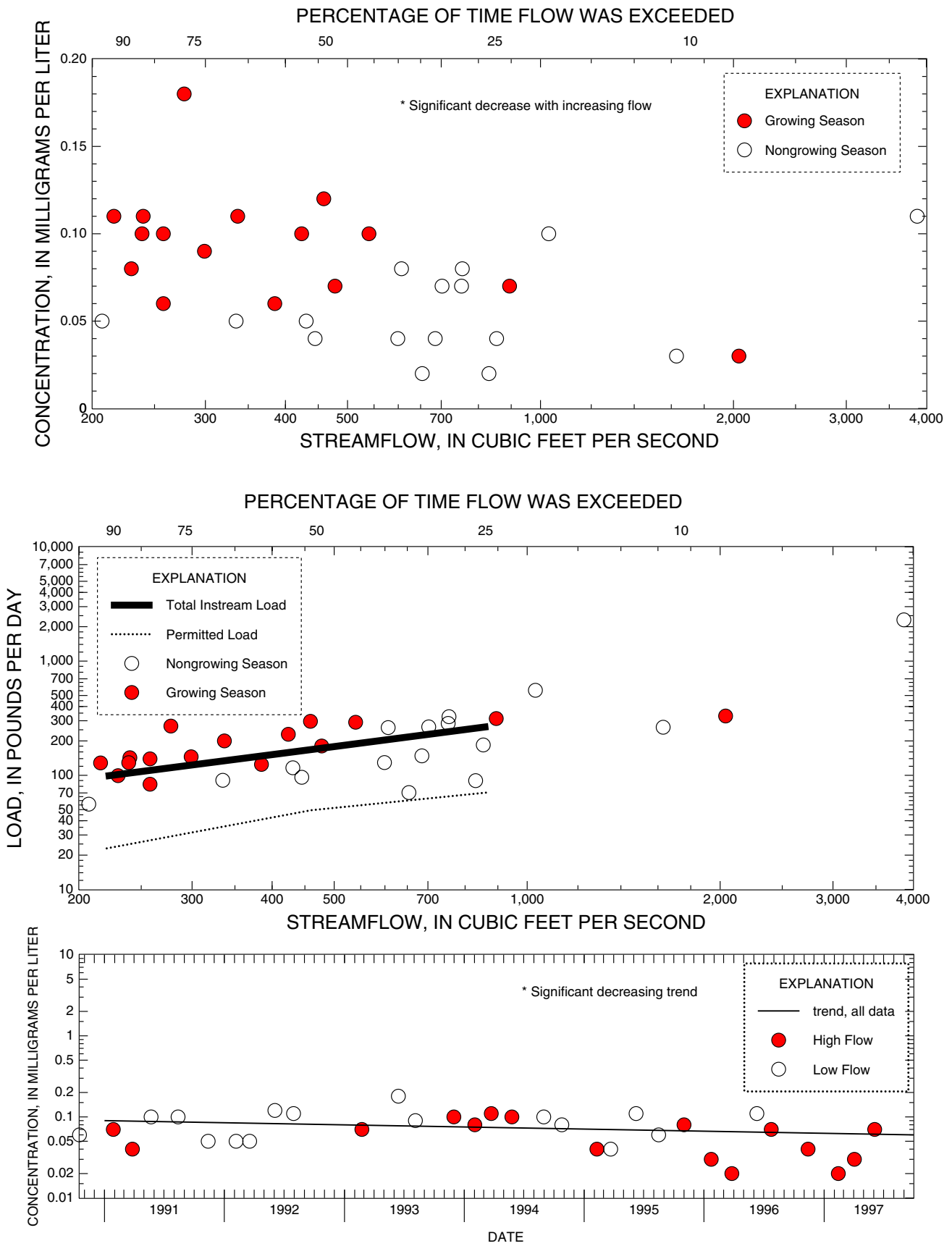
Figure F-13. Relation of total phosphorus concentrations and load to streamflow and trends in low and high-flow concentrations at 01400500 Raritan River at Manville, NJ
