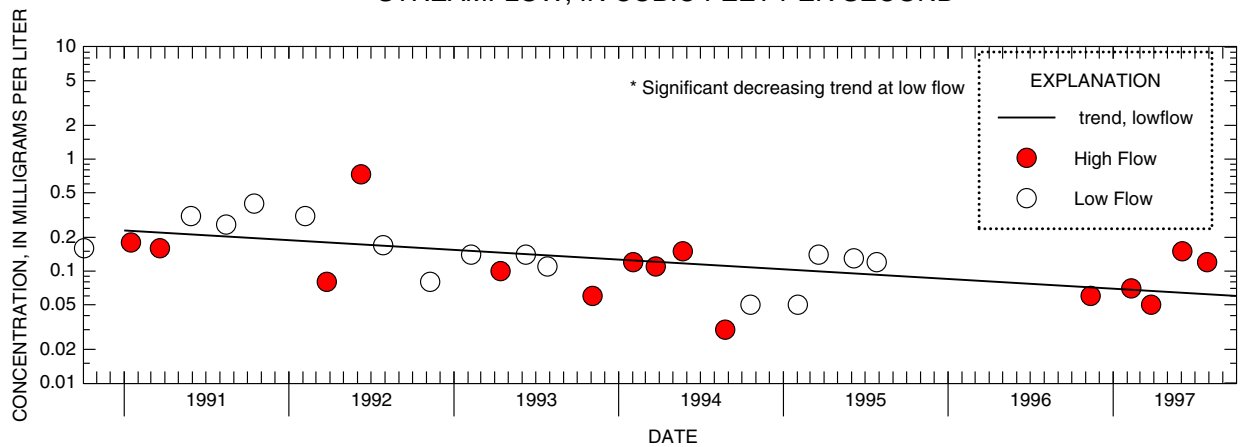
Figure F-15. Relation of total phosphorus concentrations and load to streamflow and trends in low and high-flow concentrations at 01400650 Millstone River at Grovers Mill, NJ
