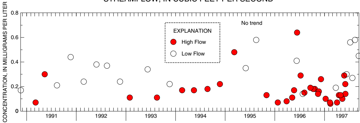
Figure F-19. Relation of total phosphorus concentrations and load to streamflow and trends in low and high-flow concentrations at 01403300 Raritan River at Queens Bridge at Bound Brook, NJ
