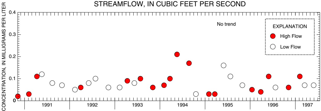
Figure F-21. Relation of total phosphorus concentrations and load to streamflow and trends in low and high-flow concentrations at 01405340 Manalapan Brook at Federal Road at Manalapan, NJ
