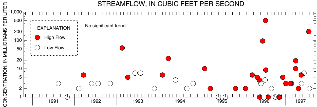
Figure G-7. Relation of total suspended solids concentrations and load to streamflow and trends in low and high-flow concentrations at 01398000 Neshanic River at Reaville, NJ
