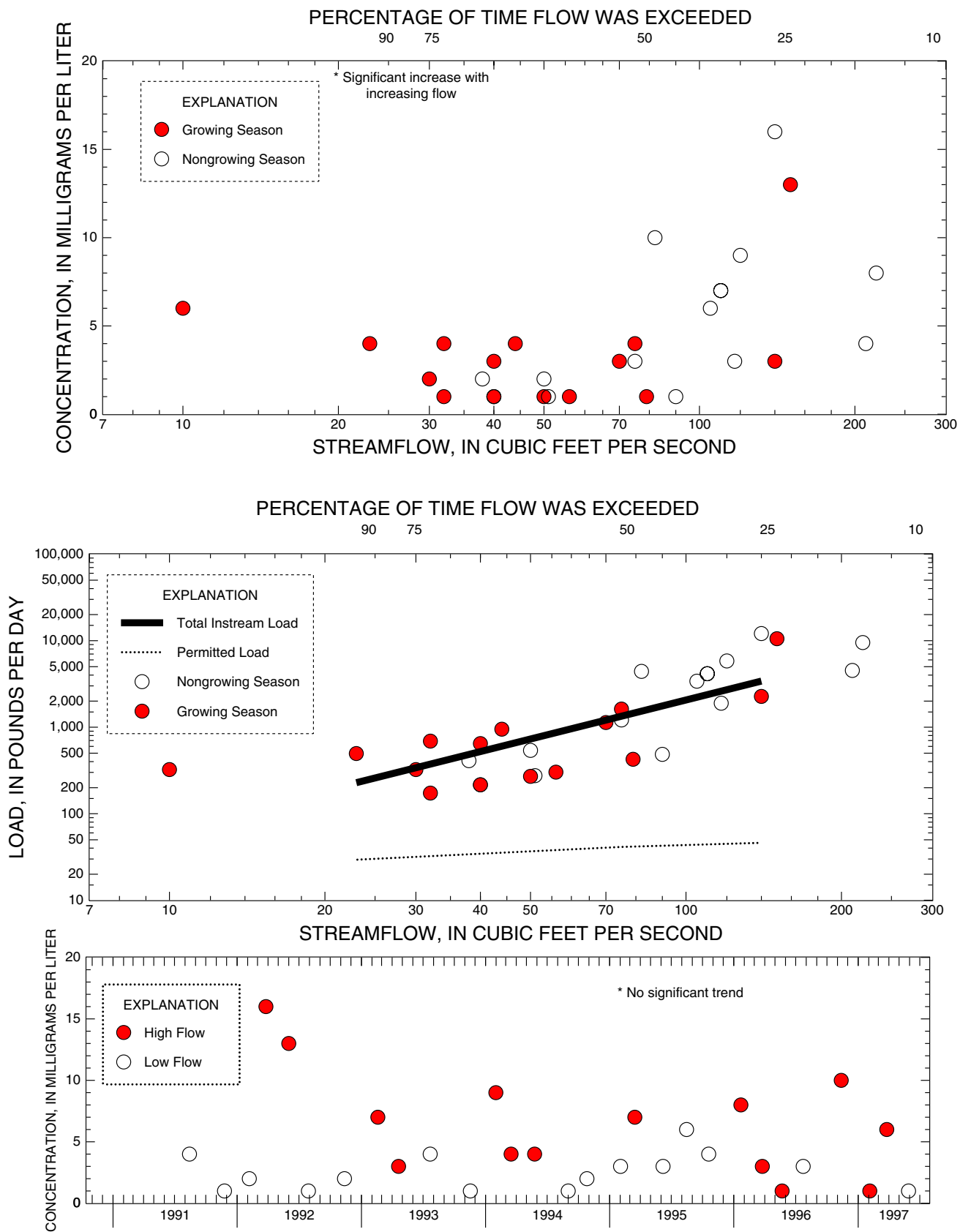
Figure G-9. Relation of total suspended solids concentrations and load to streamflow and trends in low and high-flow concentrations at 01399120 N.B. Raritan River at Burnt Mills, NJ
