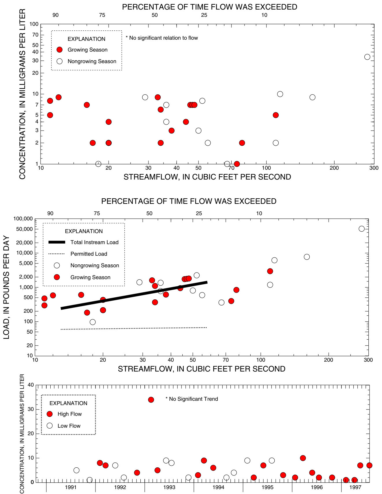
Figure G-11. Relation of total suspended solids concentrations and load to streamflow and trends in low and high-flow concentrations at 01399700 Rockaway Creek at Whitehouse, NJ
