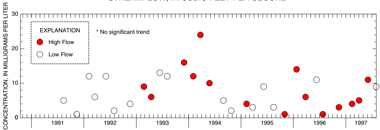
Figure G-13. Relation of total suspended solids concentrations and load to streamflow and trends in low and high-flow concentrations at 01400500 Raritan River at Manville, NJ
