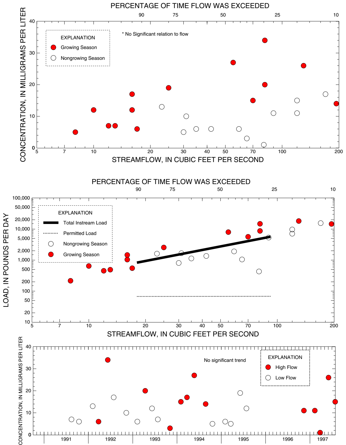
Figure G-15. Relation of total suspended solids concentrations and load to streamflow and trends in low and high-flow concentrations at 01400650 Millstone River at Grovers Mill, NJ
