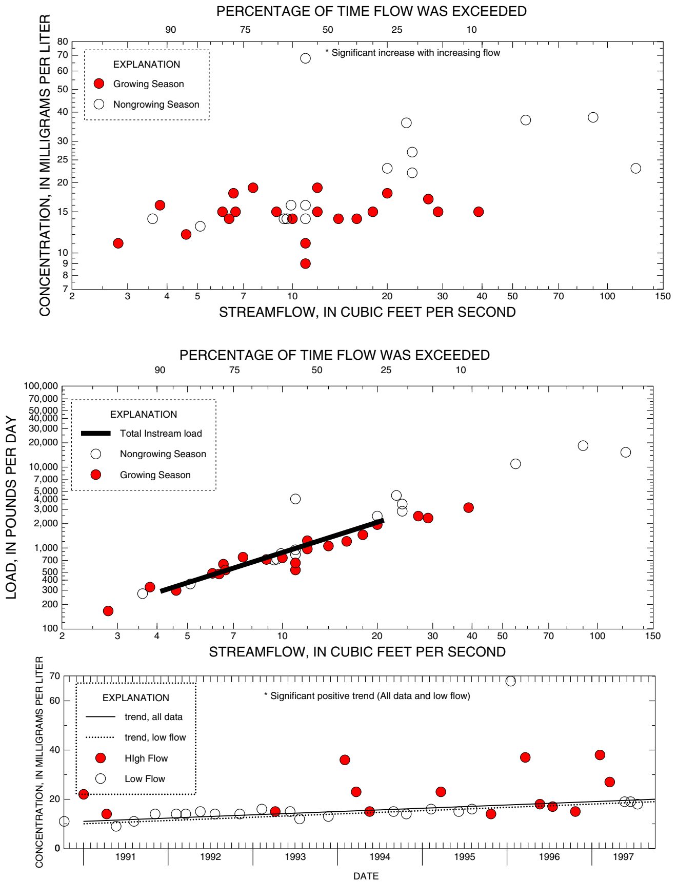
Figure H-4. Relation of chloride concentrations and load to streamflow and trends in low and high-flow concentrations at 01396660 Mulhockaway Creek near Van Syckel, NJ
