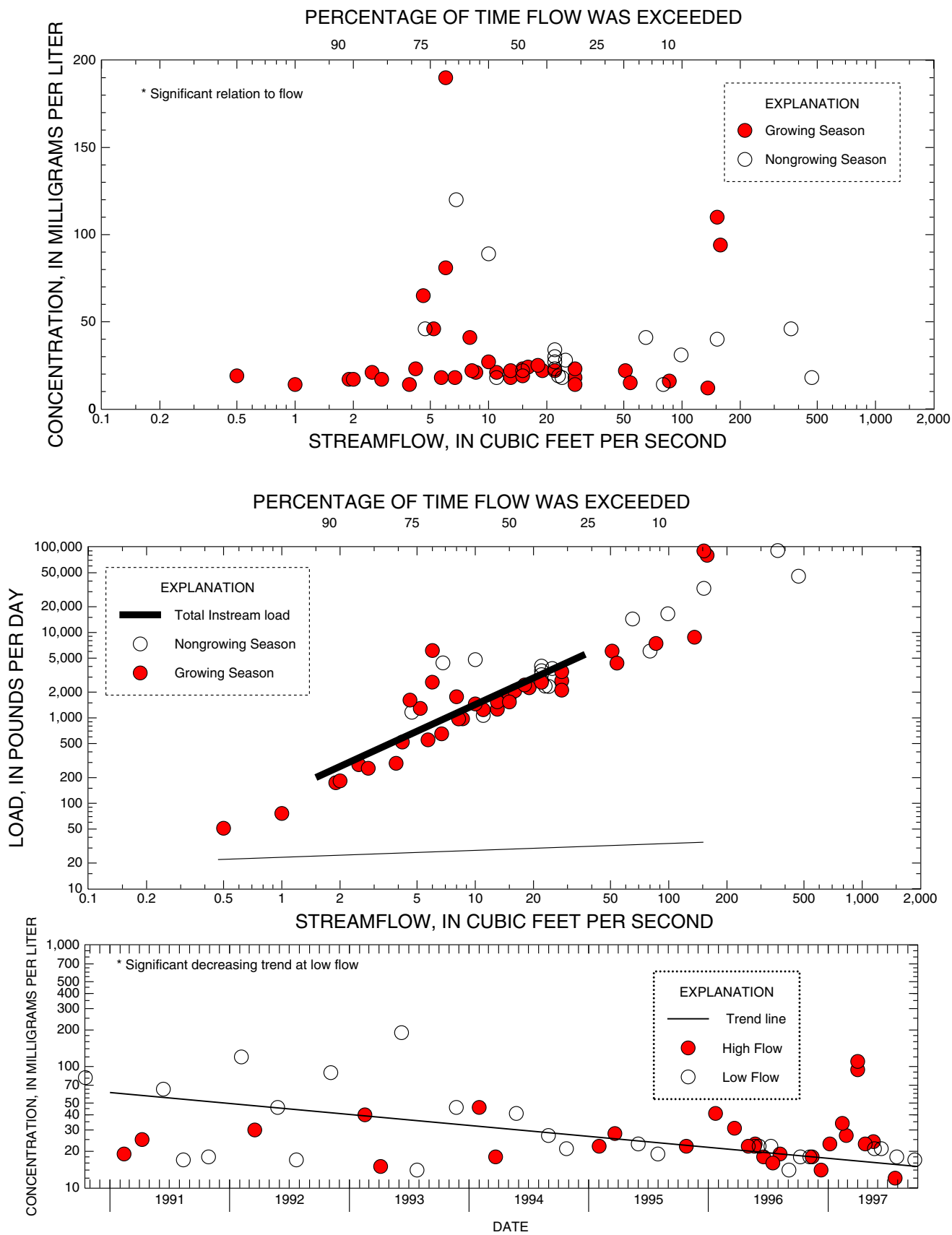
Figure H-7. Relation of chloride concentrations and load to streamflow and trends in low and high-flow concentrations at 01398000 Neshanic River at Reaville, NJ
