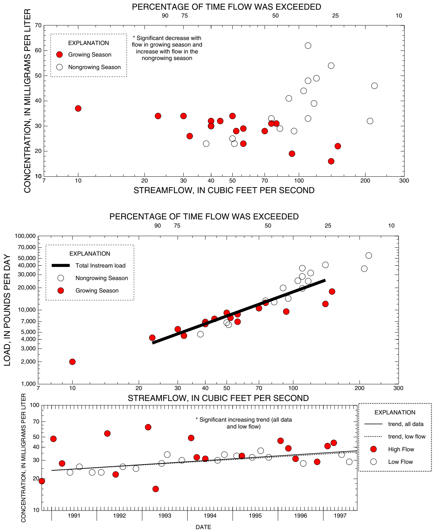
Figure H-9. Relation of chloride concentrations and load to streamflow and trends in low and high-flow concentrations at 01399120 N.B. Raritan River at Burnt Mills, NJ
