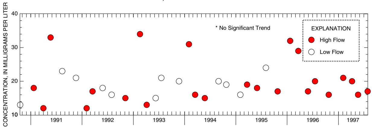
Figure H-11. Relation of chloride concentrations and load to streamflow and trends in low and high-flow concentrations at 01399700 Rockaway Creek at Whitehouse, NJ
