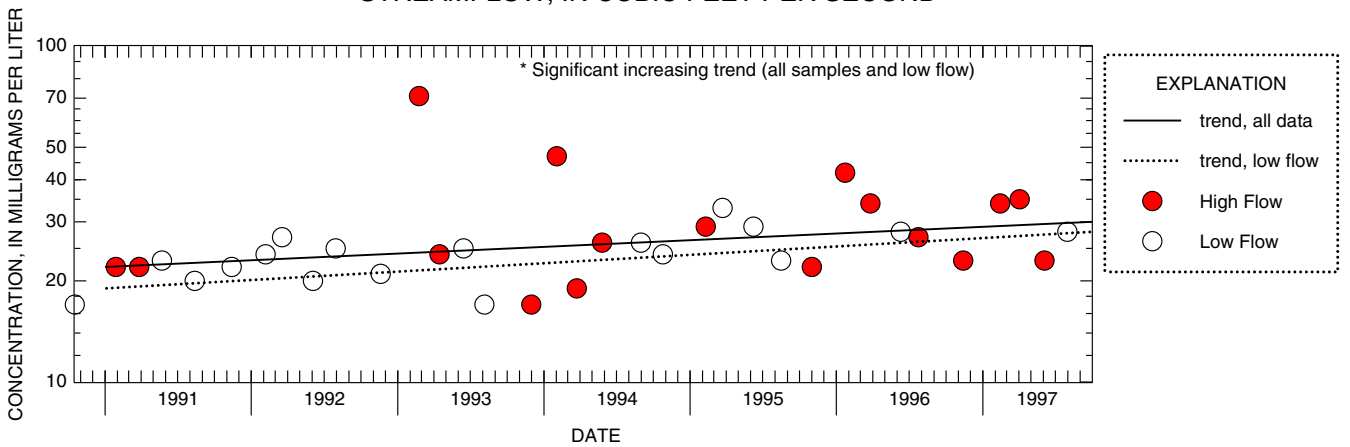
Figure H-13. Relation of chloride concentrations and load to streamflow and trends in low and high-flow concentrations at 01400500 Raritan River at Manville, NJ
