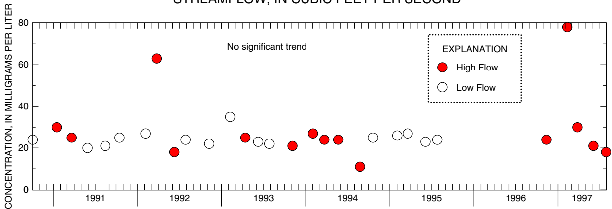
Figure H-15. Relation of chloride concentrations and load to streamflow and trends in low and high-flow concentrations at 01400650 Millstone River at Grovers Mill, NJ
