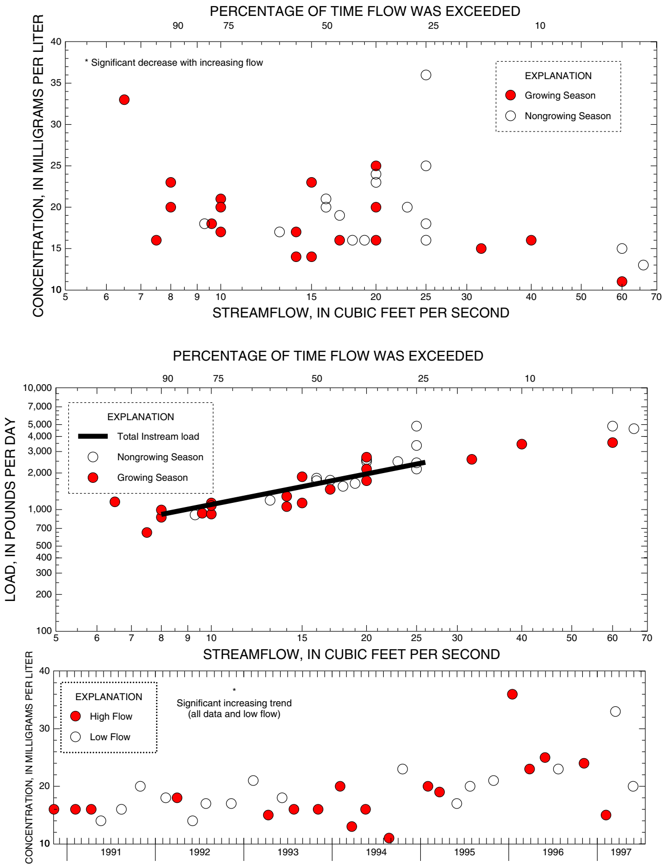
Figure H-21. Relation of chloride concentrations and load to streamflow and trends in low and high-flow concentrations at 01405340 Manalapan Brook at Federal Road at Manalapan, NJ
