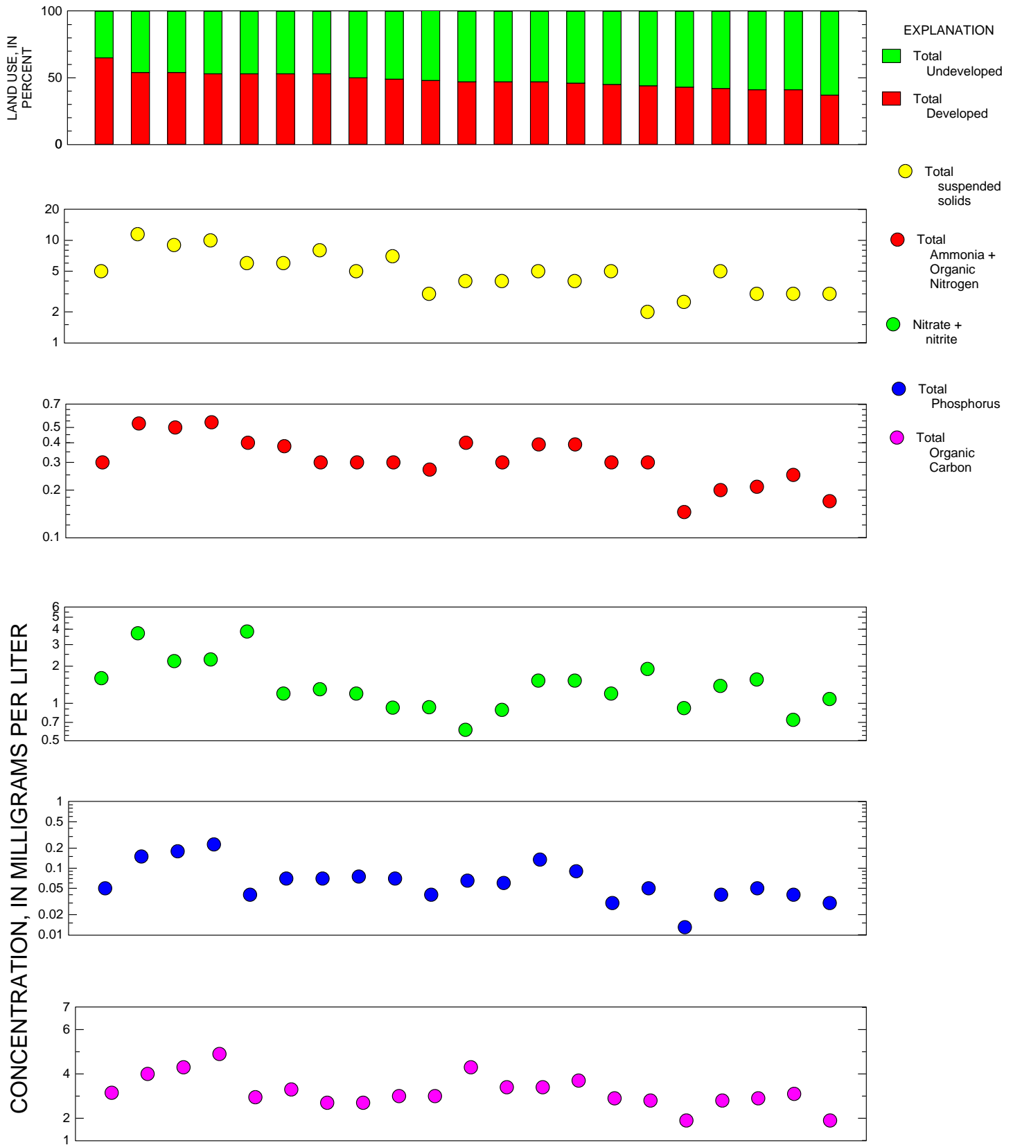
Figure 3. Relation of median concentrations of 5 constituents from samples collected from 1991-97 to percent total developed land use in the drainage basin [Five of eight constituents studied for load analysis increase with an increase in total developed land]
